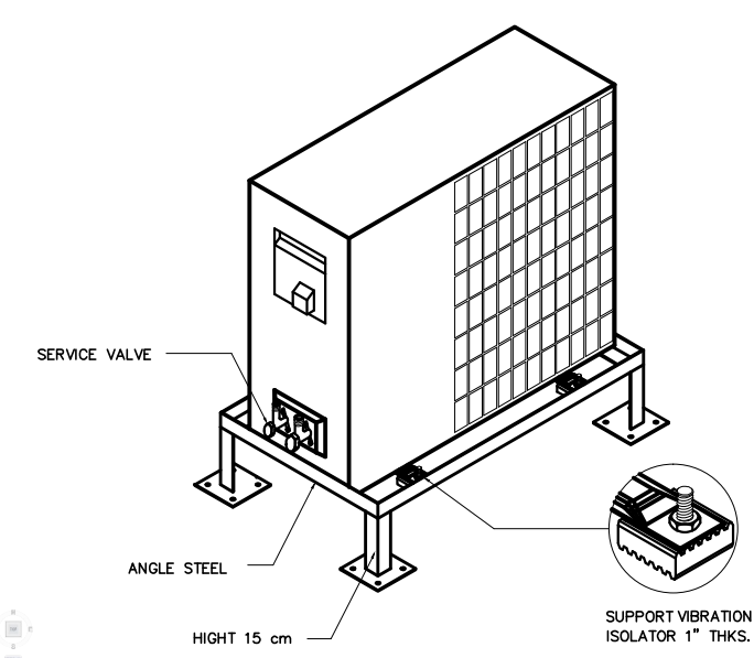
CONDENSING UNIT
