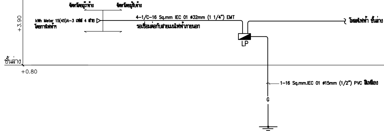
ELECTRICAL RISER DIAGRAM
