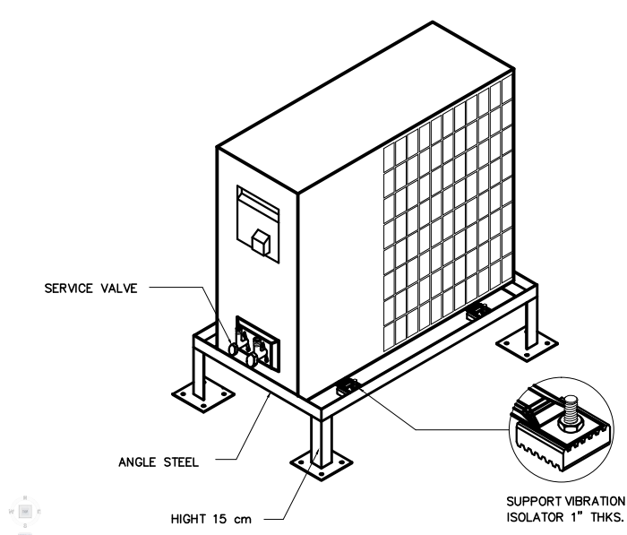
CONDENSING UNIT
