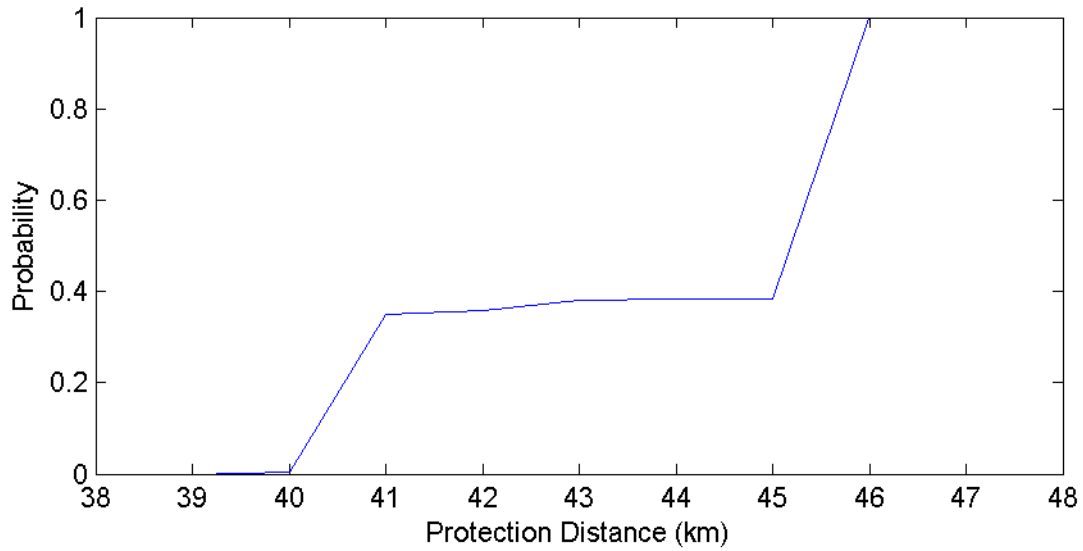
FIGURE 6 Miami Florida PEOS protection distances – 15 MHz channel (1 000 Iterations)
