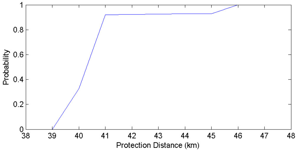
FIGURE 5 Miami Florida PEOS protection distances – 10 MHz channel (1 000 Iterations)
