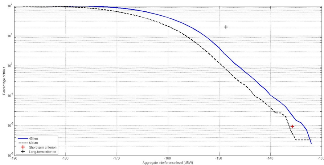
Interference cumulative distribution function from 10 MHz UEs to Lannion MetSat earth station
