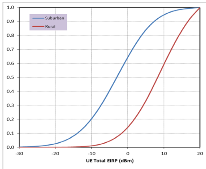
FIGURE 2 Suburban and rural UE CDF
