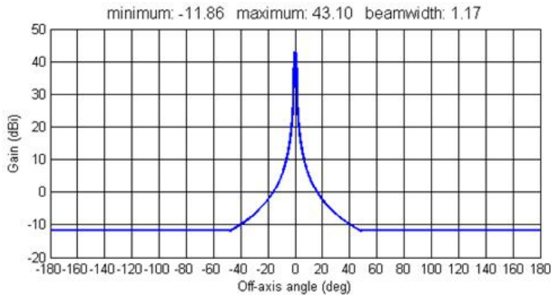
FIGURE 3 Azimuth and elevation antenna pattern
