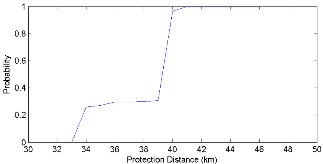
FIGURE 4 Miami Florida PEOS protection distances – 5 MHz channel (1 000 iterations)
