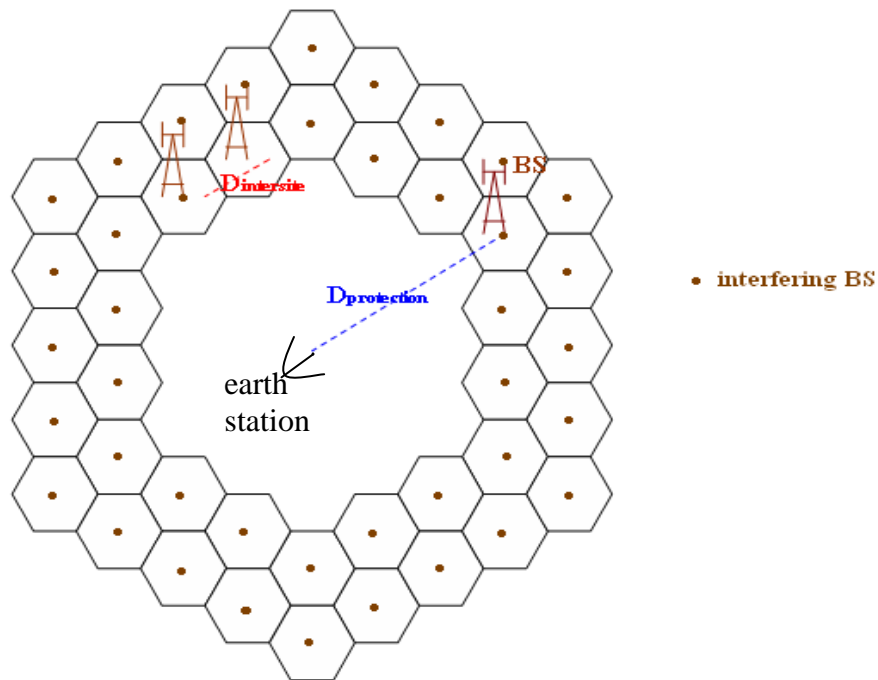
FIGURE 1 Aggregated IMT base-stations scenario
