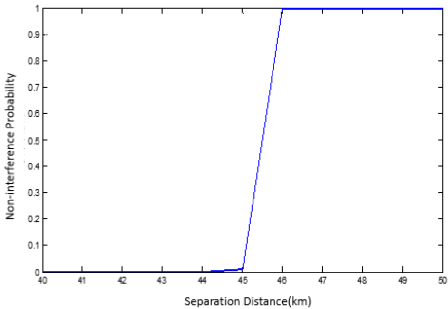
FY-4 earth station protection distances (10MHz channel bandwidth)
