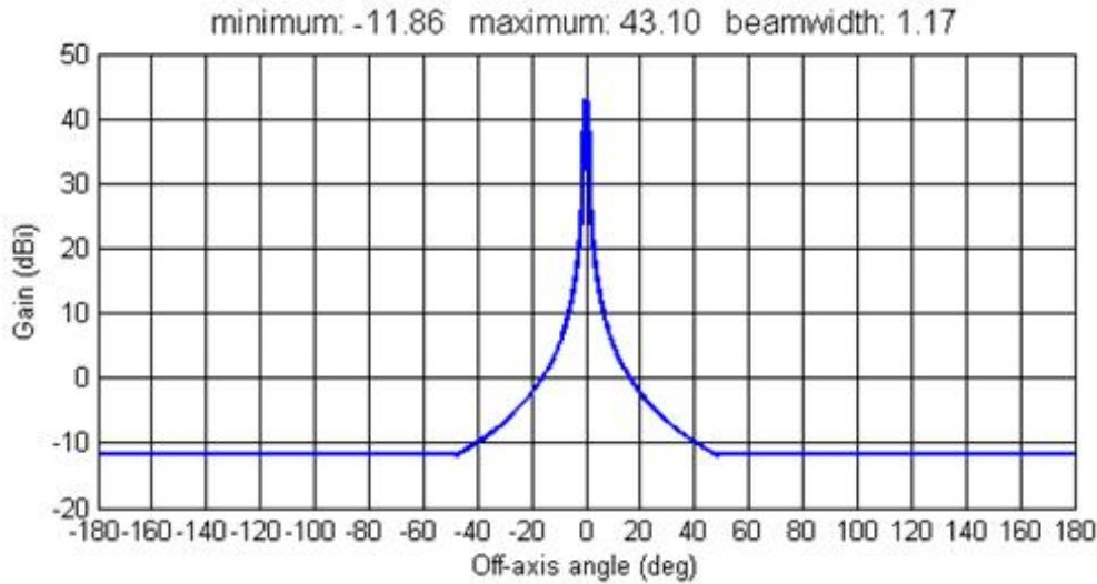
FIGURE 1 Azimuth and elevation antenna pattern
