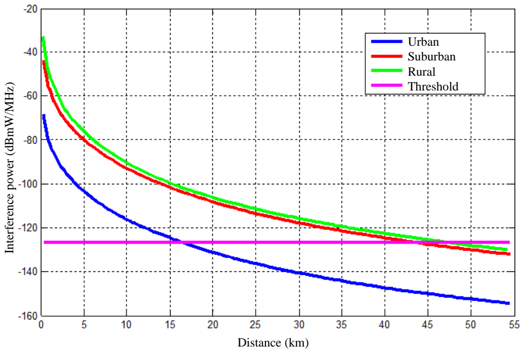
Separation distance for FY-4 earth station with single-entry interference
